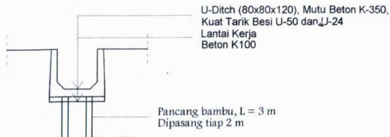
DETAIL SALURAN DRAINASE
