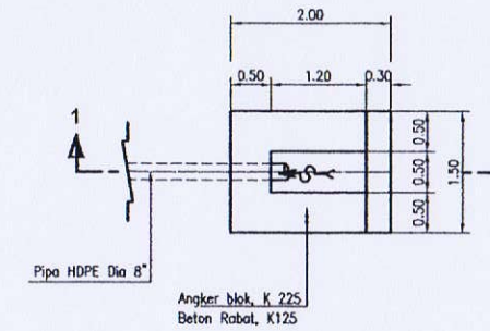
DETAIL "a" SKALA B
