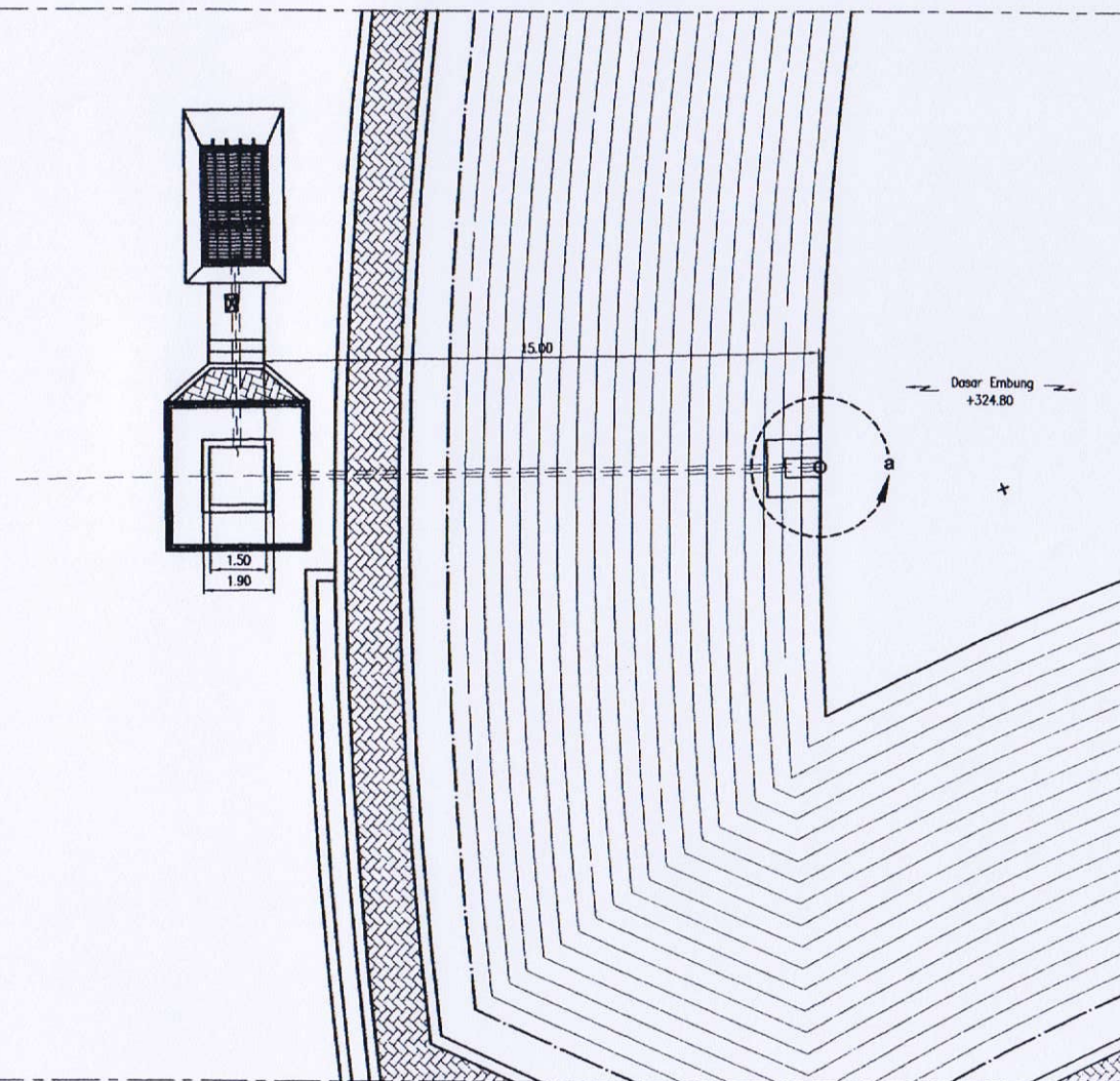
DETAIL OUTLET 1 SKALA A
